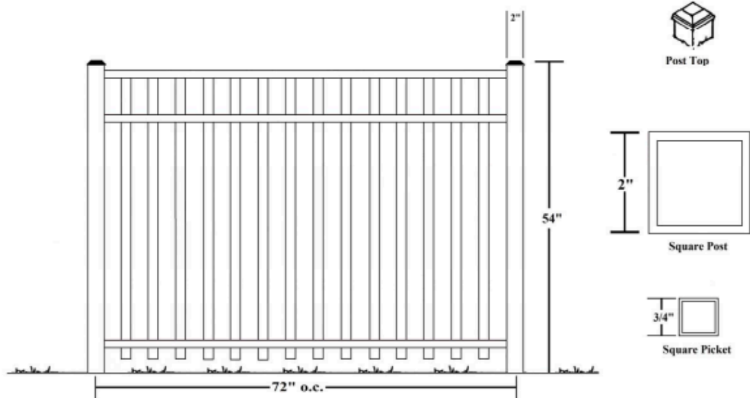
Typical Fence Detail (not to scale)
